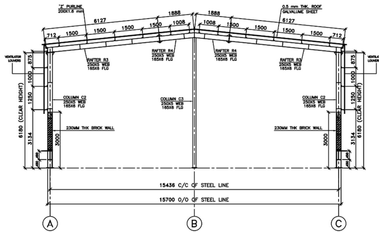
PORTAL FRAME AT GRID 1 & 5.
