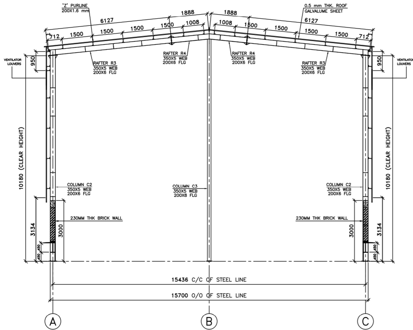
PORTAL FRAME AT GRID 1 & 5.
