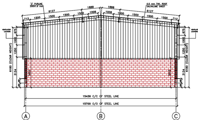
ELEVATION FOR END WALL
