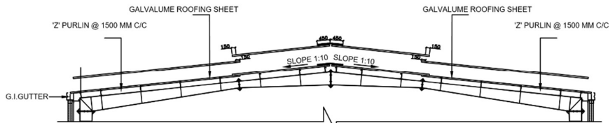
TYP. ROOF SHEETING DETAILS
