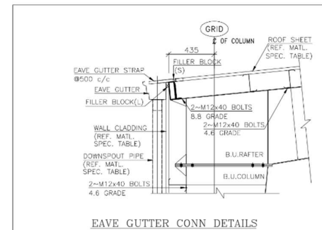
EAVE GUTTER CONN DETAILS
