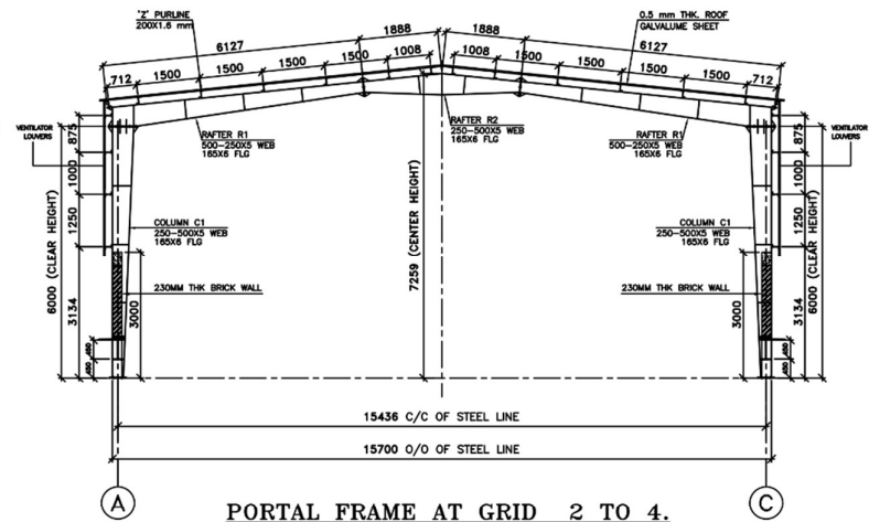
PORTAL FRAME AT GRID 2 TO 4.
